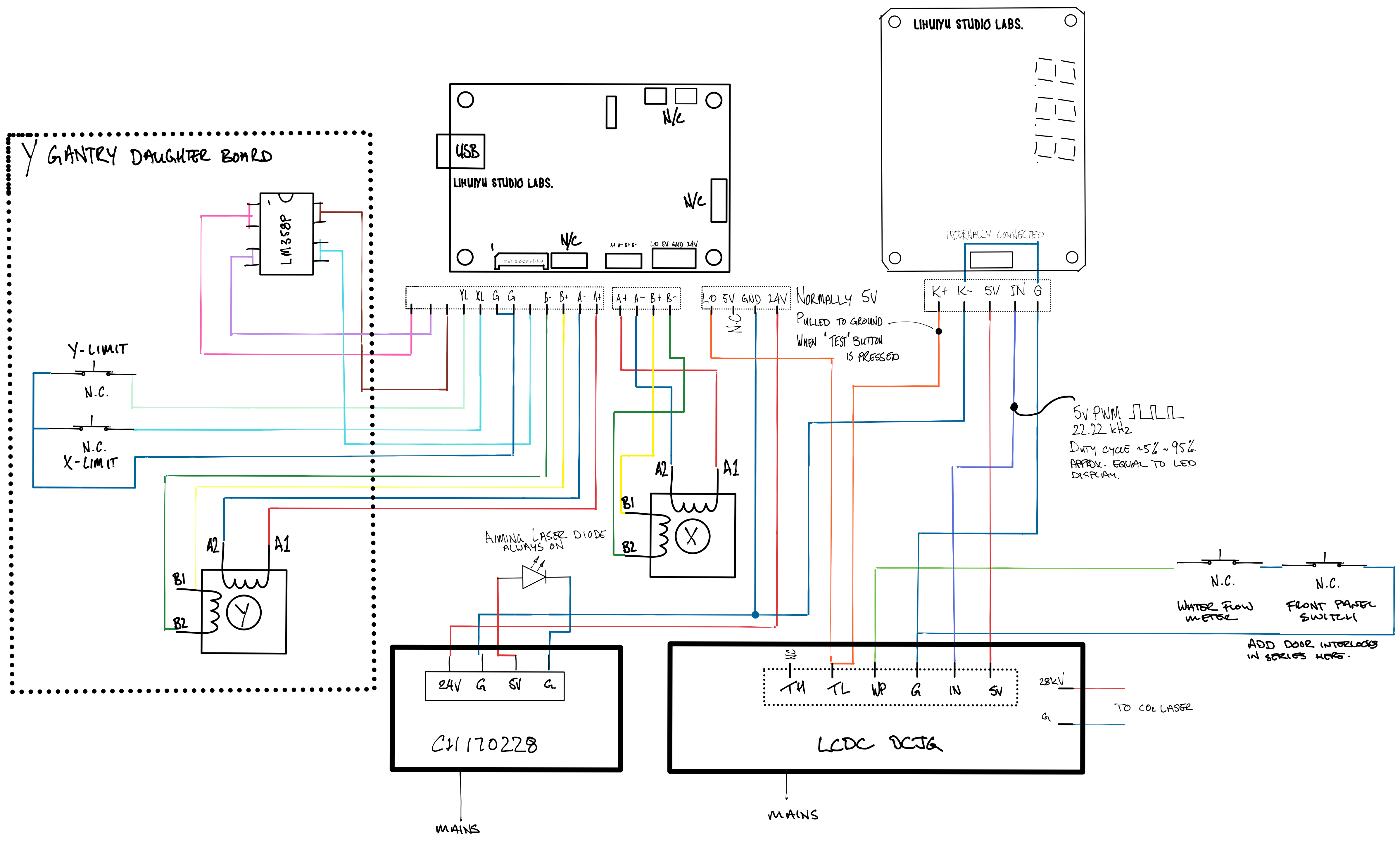
LASER CUTTER WIRING DIAGRAM REV 0
